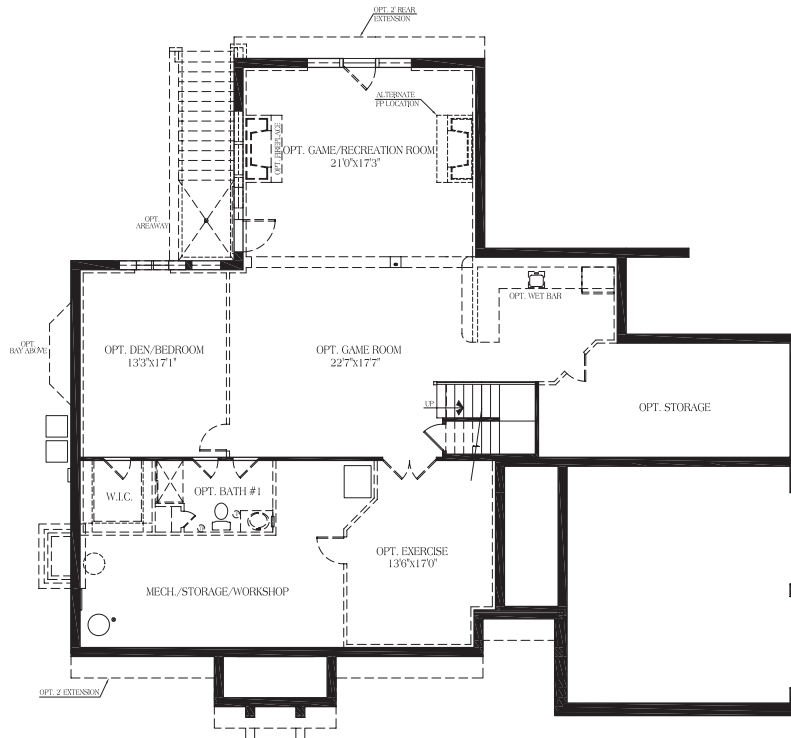
BASEMENT PLAN
