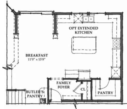
Optional extended kitchen plan
