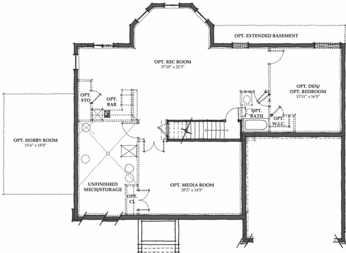
BASEMENT PLAN
