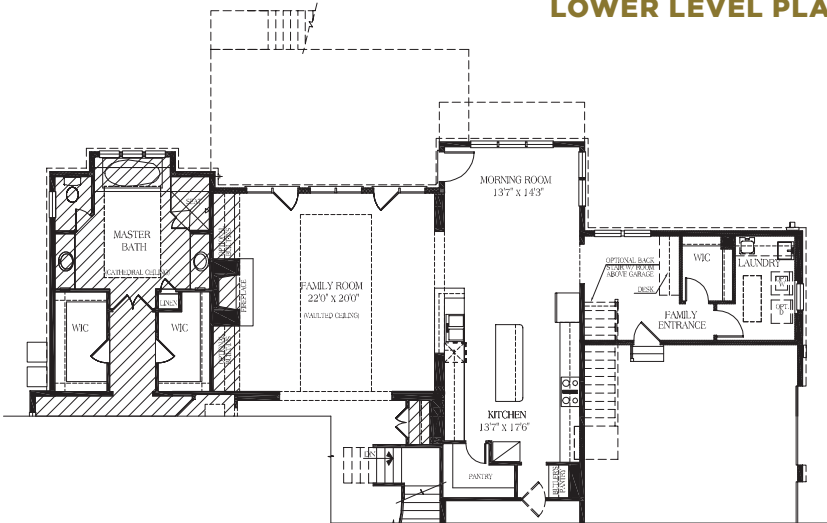
PARTIAL LOWER LEVEL PLAN with deluxe rear extension
