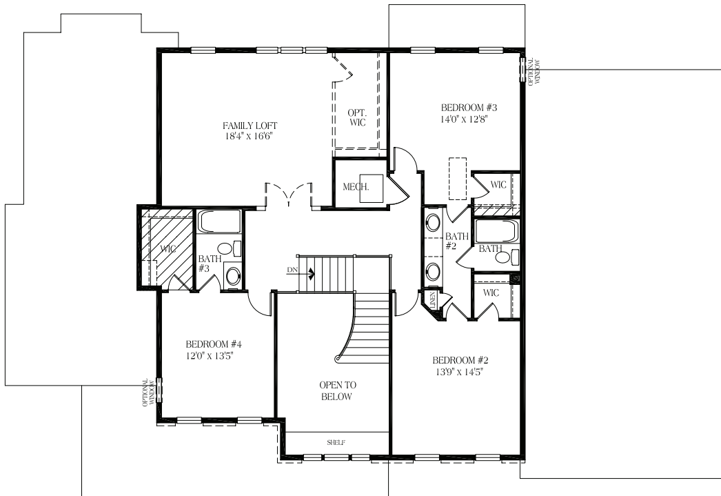
ALTERNATE UPPER LEVEL PLAN
