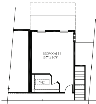
PARTIAL UPPER LEVEL PLAN with optional deluxe rear extension and optional back stair
