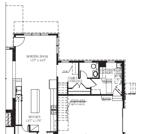
PARTIAL LOWER LEVEL PLAN with optional expanded laundry room (only available with deluxe rear extension)
