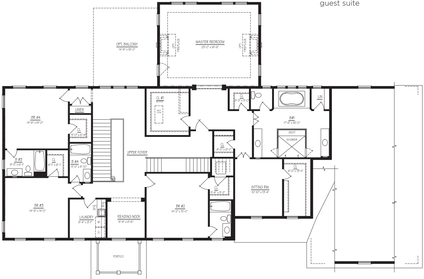
UPPER LEVEL PLAN
