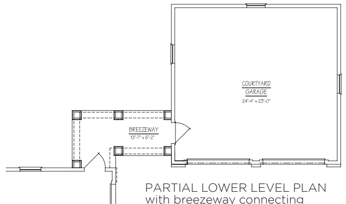
PARTIAL LOWER LEVEL PLAN with enclosed breezeway connecting to courtyard garage
