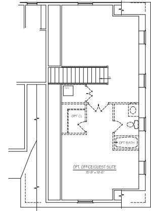
PARTIAL UPPER LEVEL PLAN with optional office/guest suite
