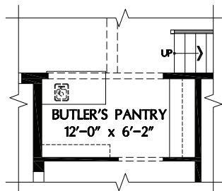
Optional Butler's Pantry
