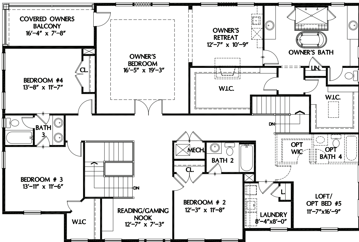
UPPER LEVEL PLAN
