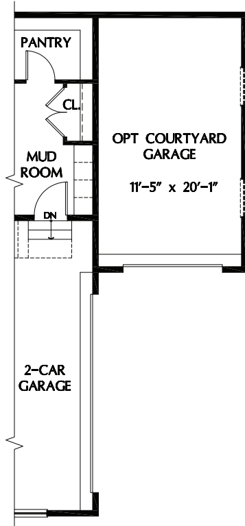
Optional 3-Car Front Load Garage
